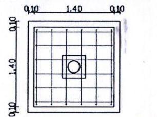
PLAN OF FOOTING
