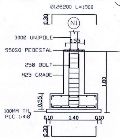
SECTION OF FOOTING
